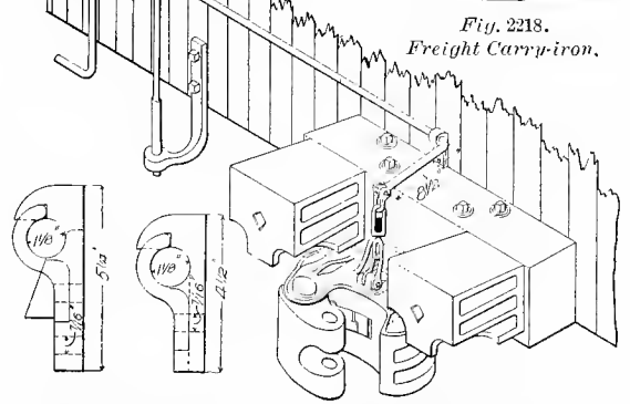
Figs. 2219-2220. Uncoupling Rod Brackets. Perspective View, showing application of Coupler.
